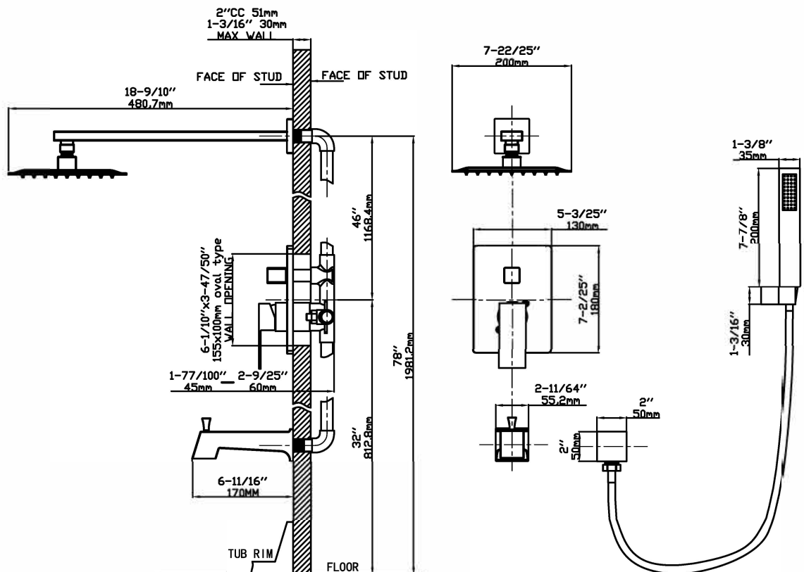
CRITICAL DIMENSIONS
