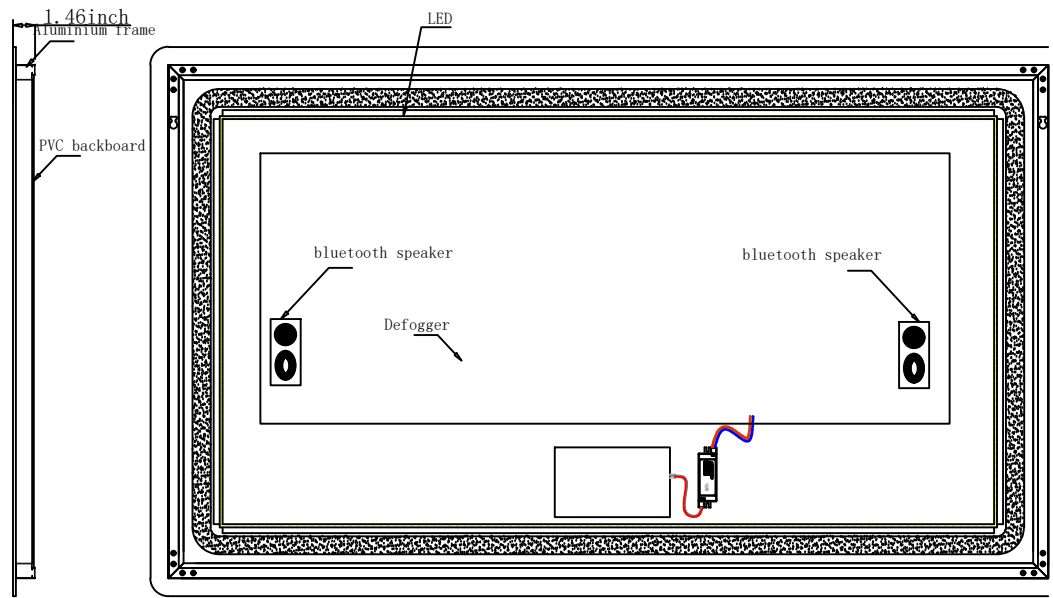
Side View
