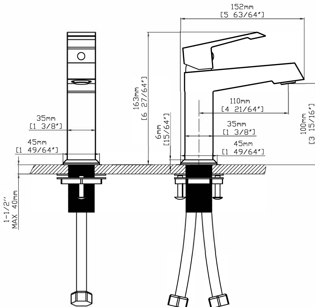
CRITICAL DIMENSIONS
