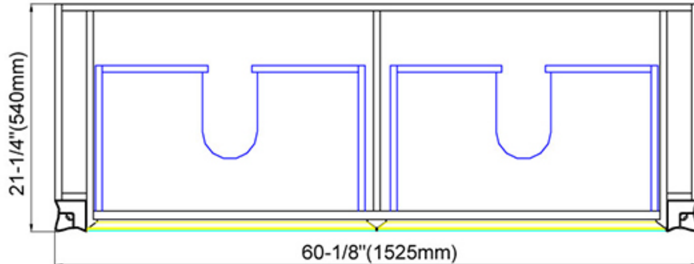
Top view
