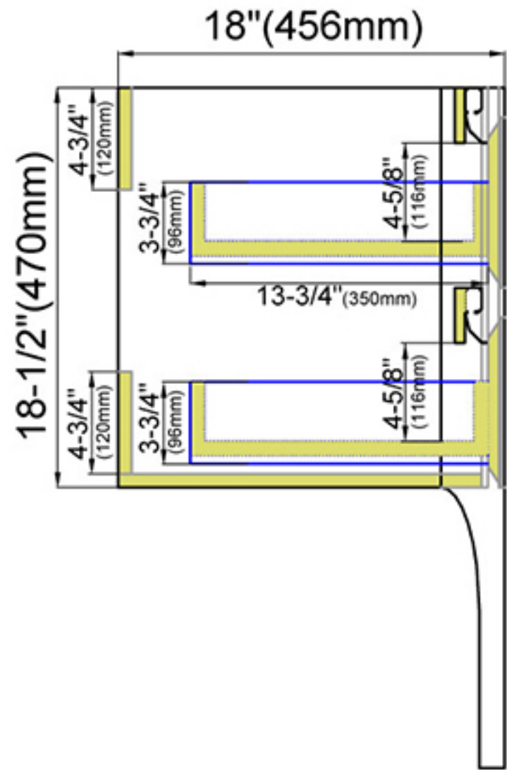
Side view
